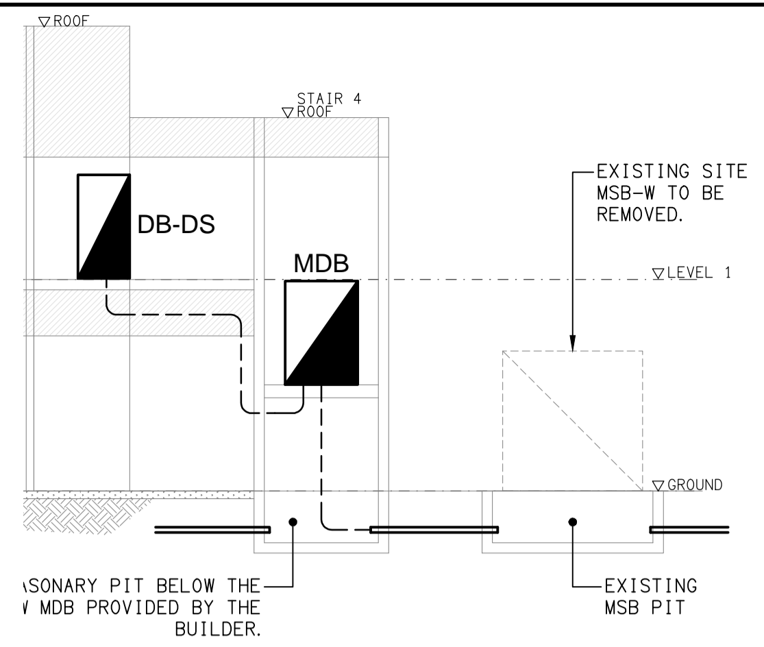
DETAIL B CABLE ROUTE SECTION NOT TO SCALE
